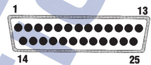
D25 Male Connector (front view)
